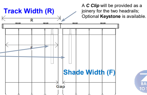
Wands at the center will be behind fabric vanes to minimize gaps.
